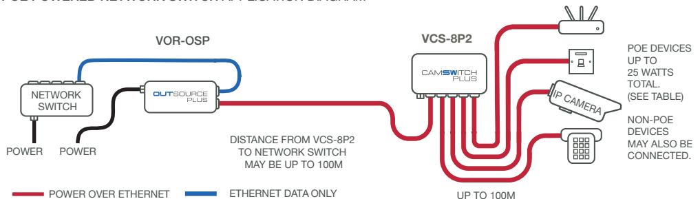
POE POWERED NETWORK SWITCH APPLICATION DIAGRAM
