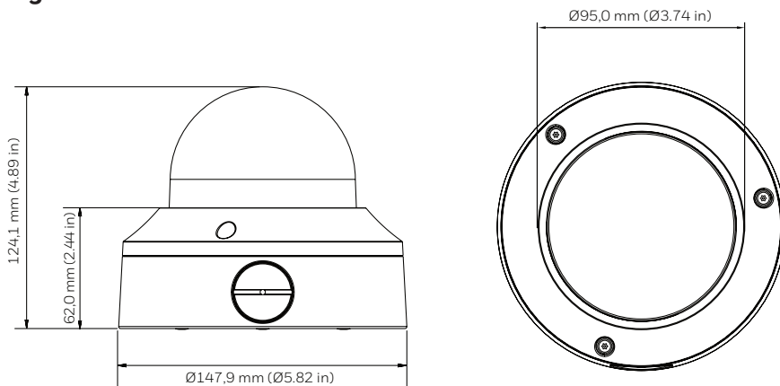
Figure 1. Dimensions
