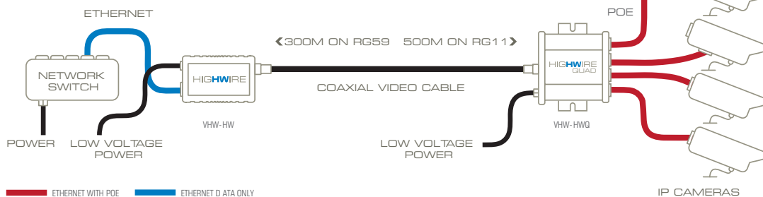
Diagram 2. A single HIGHWIRE combined with a HIGHWIRE Quad provides Ethernet connectivity for up to four POE IP devices (typically IP cameras) over existing coaxial cabling.
