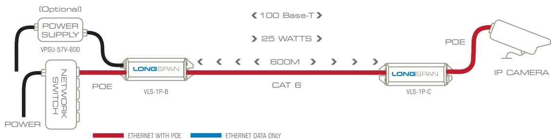
Diagram 1. A pair of LONGSPAN converters deliver full-bandwidth Ethernet & optional full-power POE over greatly extended distances of regular network cable or UTP.
